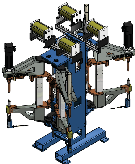
FlexFast Acrobat with Four arms, four projection weld set-ups & four transformers
