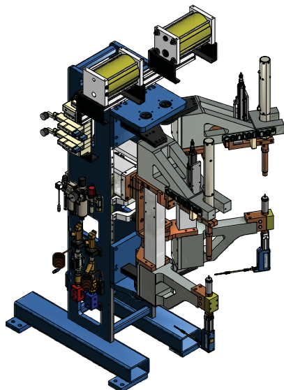
FlexFast Acrobat with two arms, air/oil weld actuators, dual transformers.
