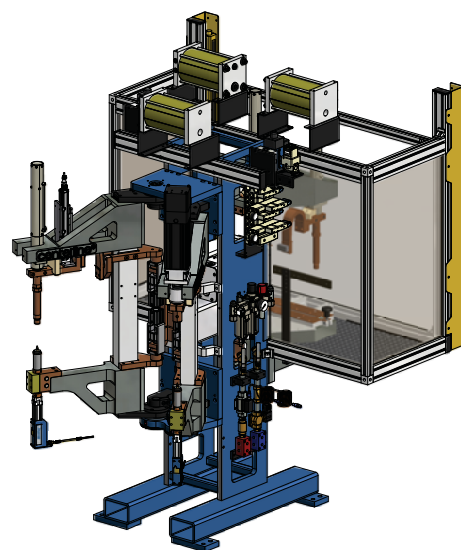
FlexFast Acrobat with two arms, one cell & three transformers
